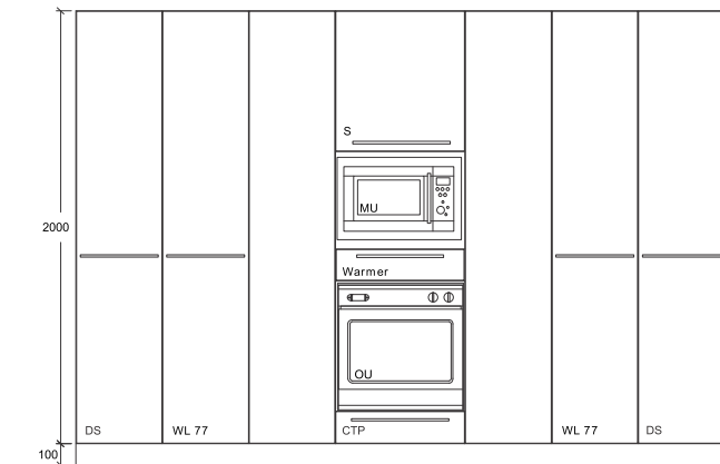
ELEVATION 'A'
