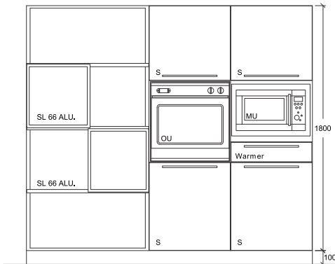
ELEVATION 'A'
