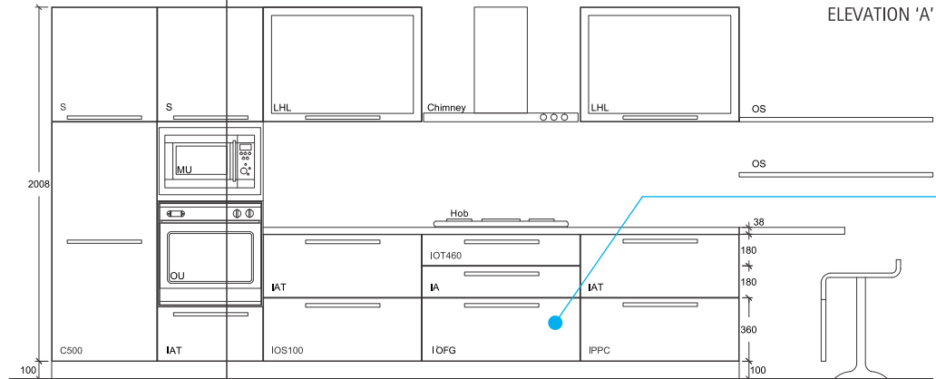
ELEVATION 'A'
