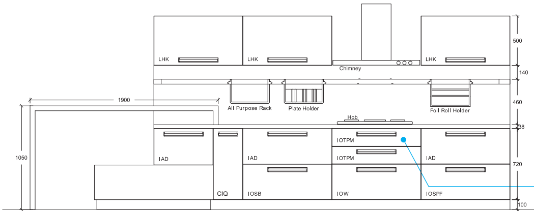
ELEVATION 'A'
