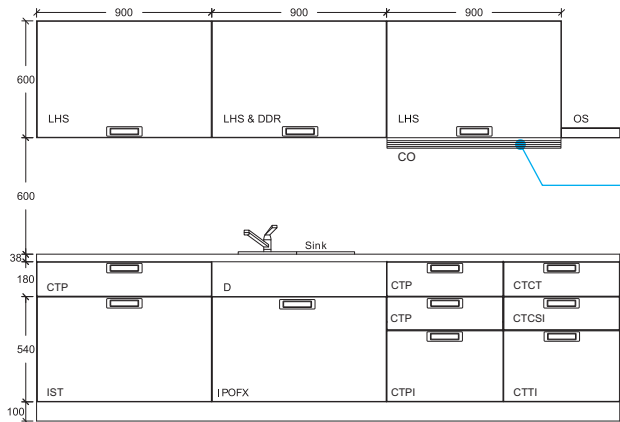
ELEVATION 'A'
