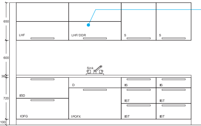
ELEVATION 'A'
