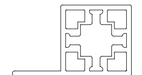
Profile for side/shelf panels 16mm
