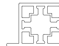
Profile for shelf panels 16mm
