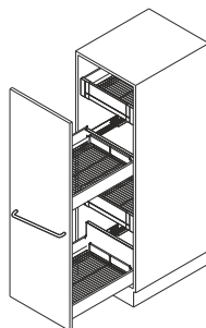
For carcass width 450 mm
