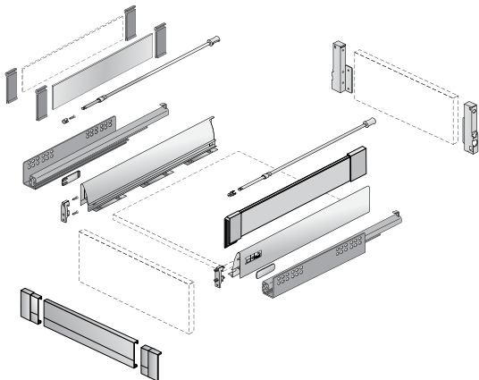
Drawer set 70 mm height
