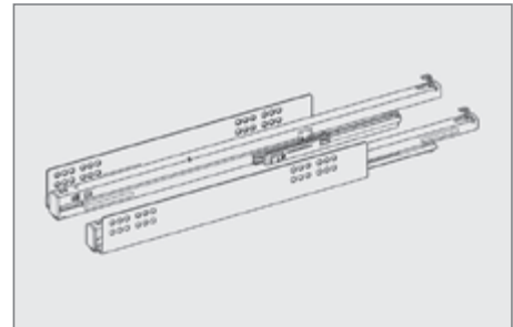
Full extension runner, Quadro V6+ Load capacity up to 50 kg ► with Silent System or Push to open
