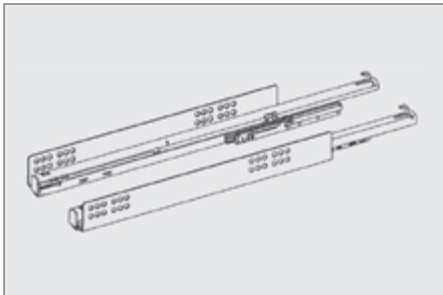
Quadro V6 full extension runner Load capacity up to 30 kg ► with Silent System or Push to open
